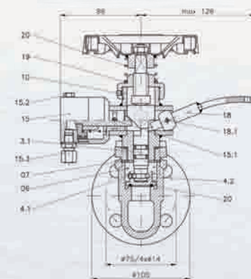
Selbstschlussventil, hydr./pn. anlüftbar self-closing valve, hydr./pn. liftable
